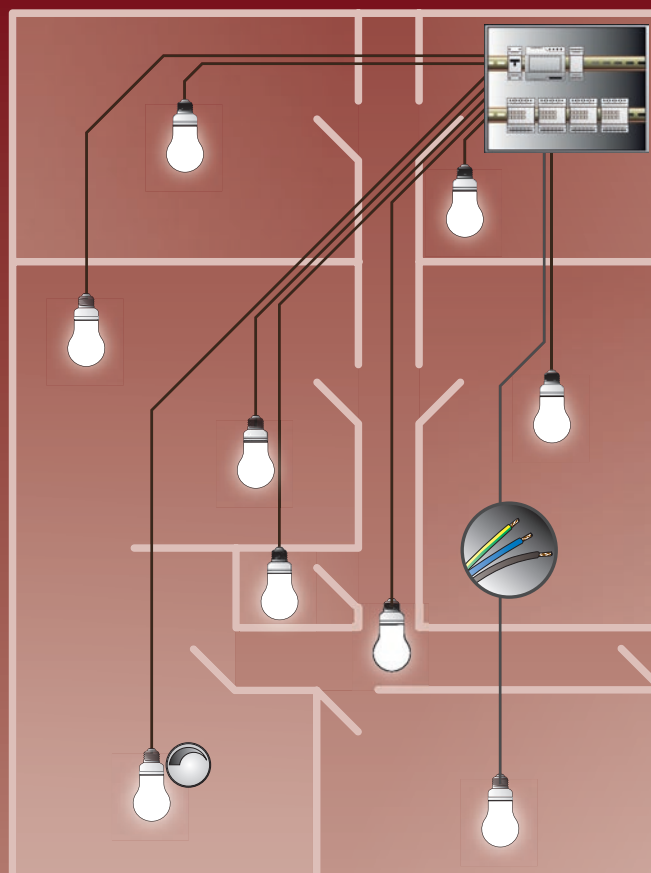
230V WIRING 8 light points + 1 dimmable
