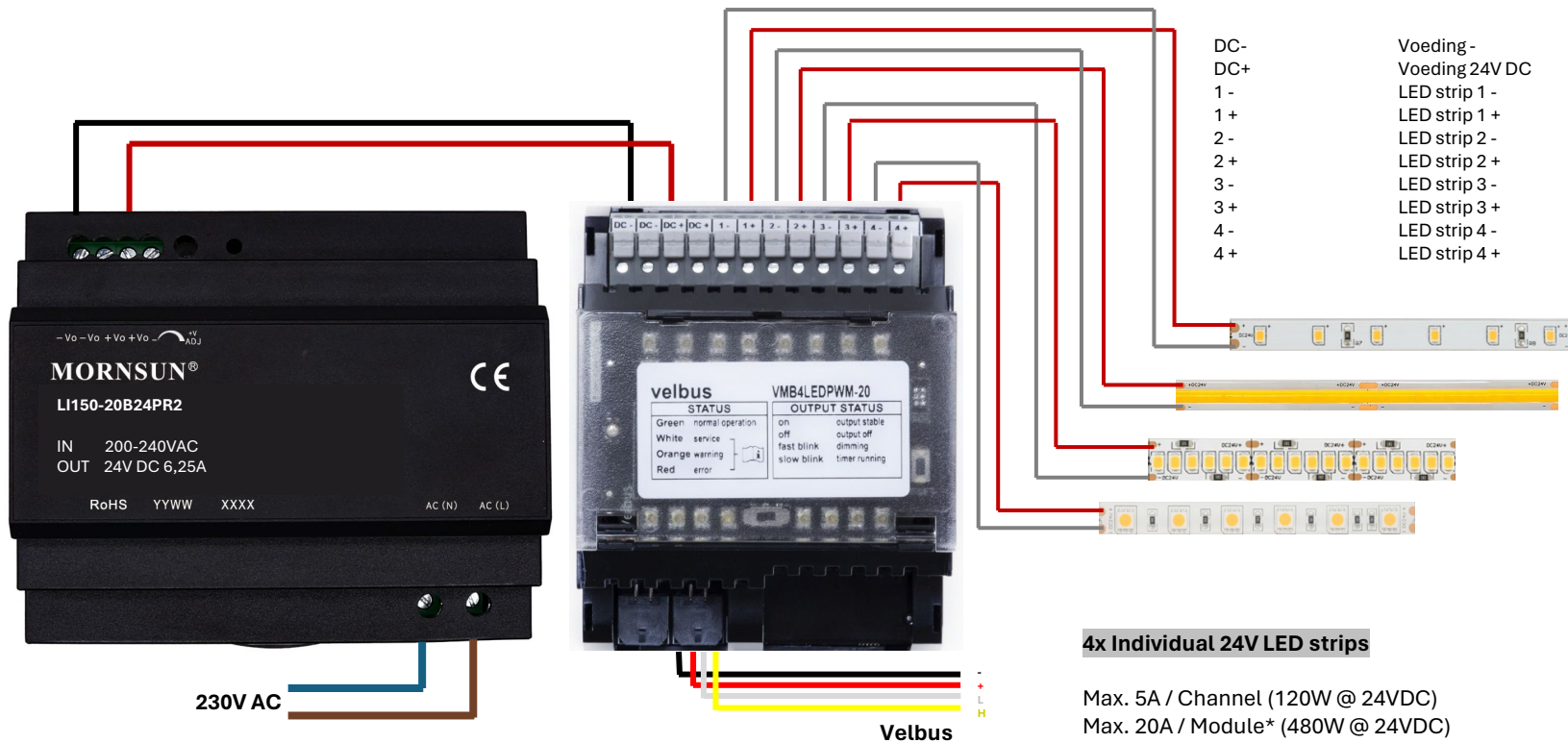
LI150-20B24PR2 Power supply 24V DC – 150W
